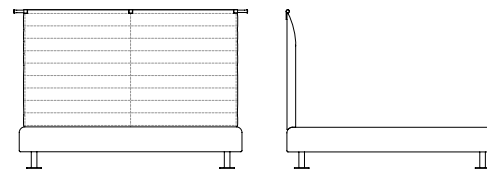
50054 + 50051 Giroletto + Testata imbottita alta Bed frame + High upholstered headboard cm 208 x 218 x h 146 in 81 7/8 x 85 7/8 x h 57 1/2 RETE - SLAT BASE cm 180 in 70 7/8
